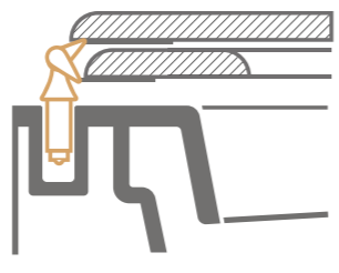
Attacco verticale con vite e tassello ad espansione Vertical attachment with screw and expansion plug
