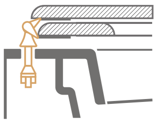
Attacco verticale con vite passante a galletto Vertical attachment with through wing nut
